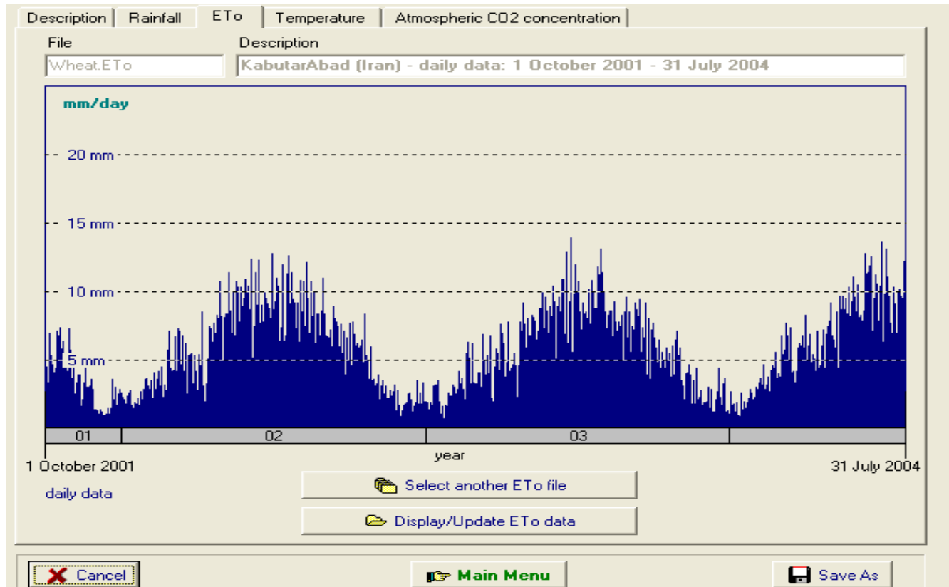
Figure 2. ET 0 computed from daily meteorological data using the PM equation (2001 to 2004).
